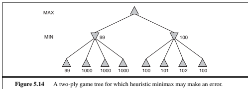
Figure 5.14 A two-ply game tree for which heuristic minimax may make an error.
