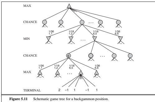
Figure 5.11 Schematic game tree for a backgammon position.
